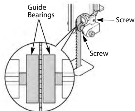
Figure 15 - Adjusting the guide bearings.
