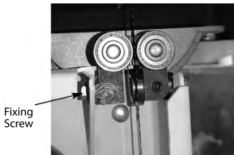
Figure 16 - Basic alignment.
