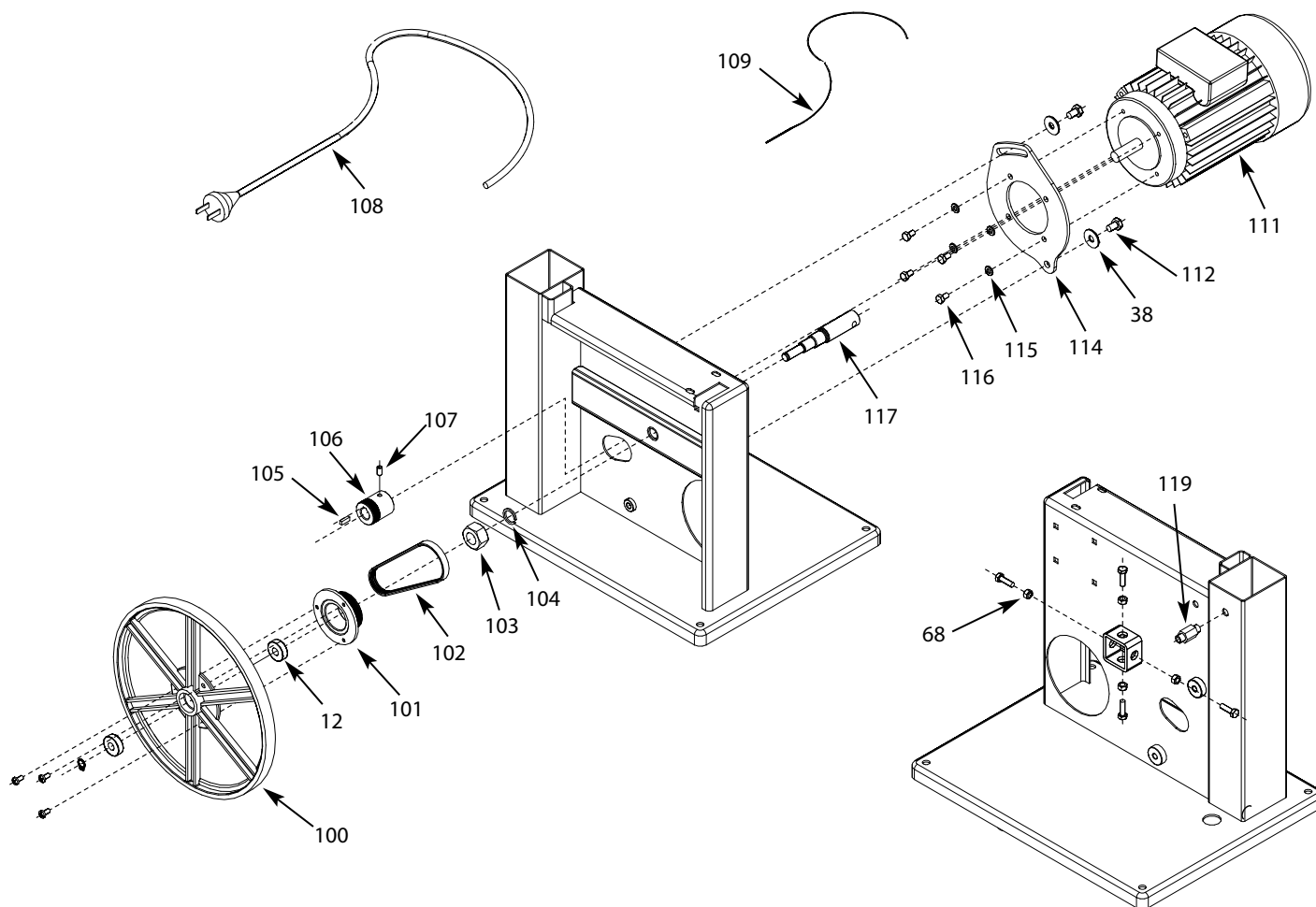
Figure 22 - Replacement parts illustration for 10" Bench Top Band Saw (continued).
