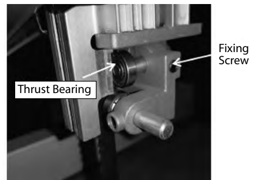
Figure 14 - Adjusting the thrust bearings.
