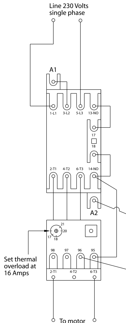
Figure 6 – Schematic
